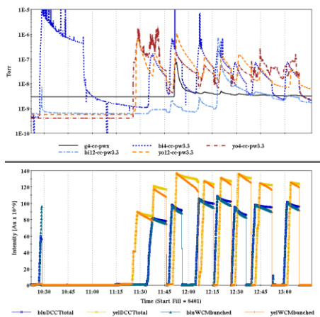
Figure 2: Pressure readings in IR4 and IR12 (top) and injected total beam current (bottom) during the scrubbing procedure.
