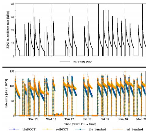
Figure 4: The best week in Run-7. Collision rates (top) and total beam current (bottom). The integrated luminosity during this week reached 380 \mu b^{-1} per experiment.
