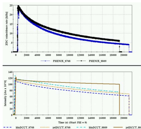
Figure 3: Beam intensity (bottom) and collision rates (top) in 2 stores with (8768) and without (8809) yellow stochastic cooling.
