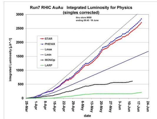
Figure 1: Integrated delivered luminosity for the four IRs with the minimum and maximum predictions up to June 19, 2007.
